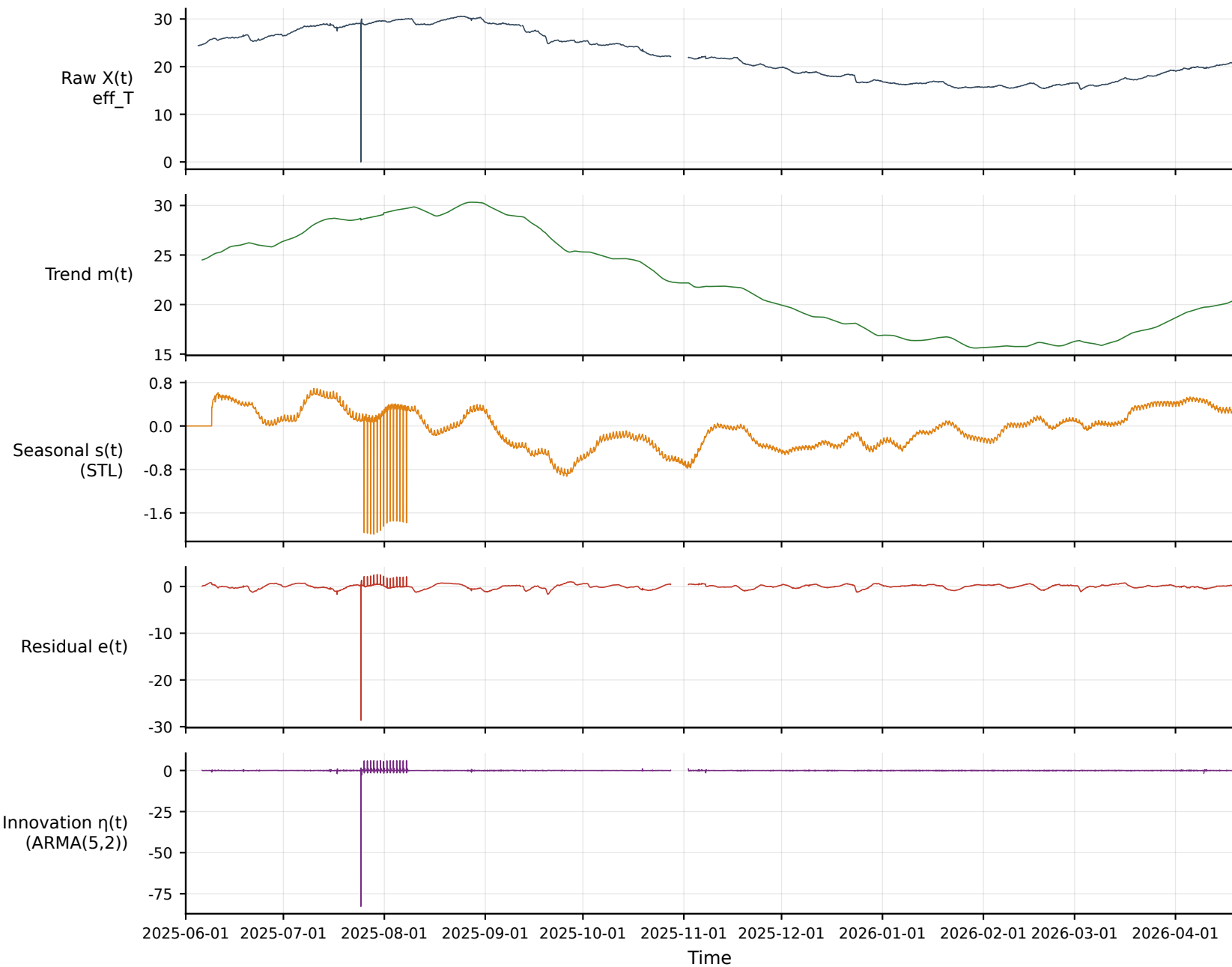
Multi-scale decomposition — eff_T (effluent, hour) [2025-06-01~2026-04-19]
